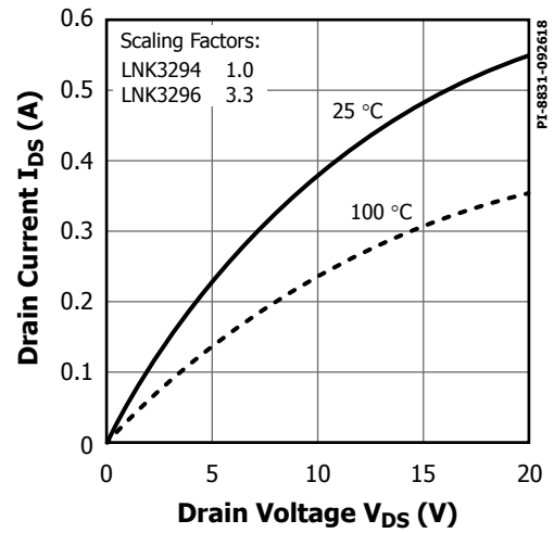
Figure 24. Output Characteristics.
